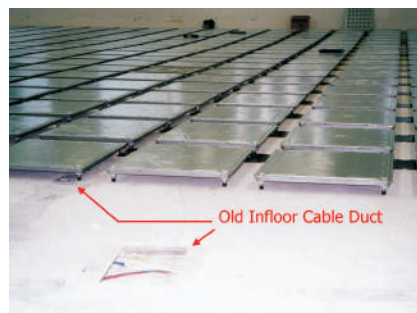
Renovation jobs: Installing on the old, embed floor trunkings
