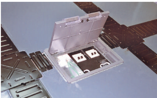
To accommodate large size floor box - Cut at side of the panel (count in the Cable Trench width) and installed at the trench.
